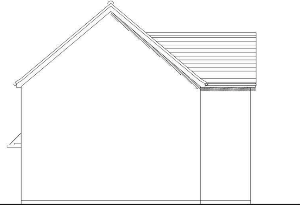
Side Elevation
